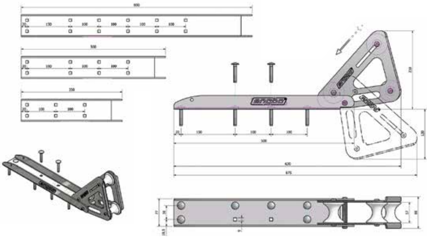
Pivoting anchor roller
