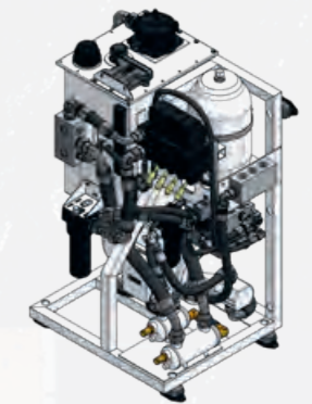
Illustration of rack assembly version for stabilizers and hydraulic thrusters
