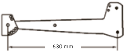
Anchor roller 61-30005
