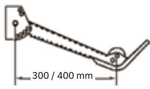
Stern anchor roller 61-30006, 61-30007
